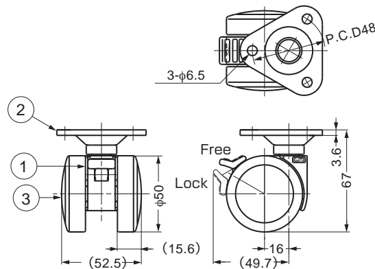
The drawing above show the model with Brake
