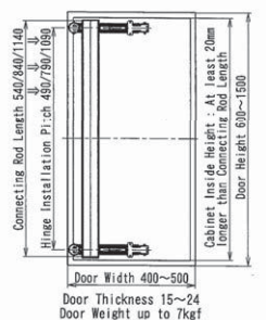
2 Hinges per door ①Damper and Catch Hinges : 2 pcs
