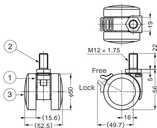
The drawing above show the model with Brake
