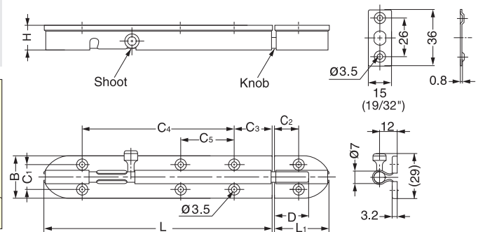
BS-240
