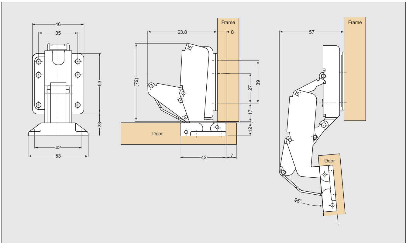
HT-160THV2
