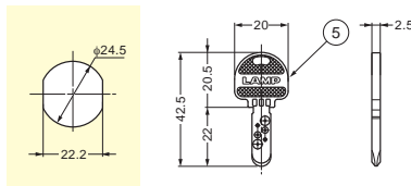
■ Cut Out Dimensions
