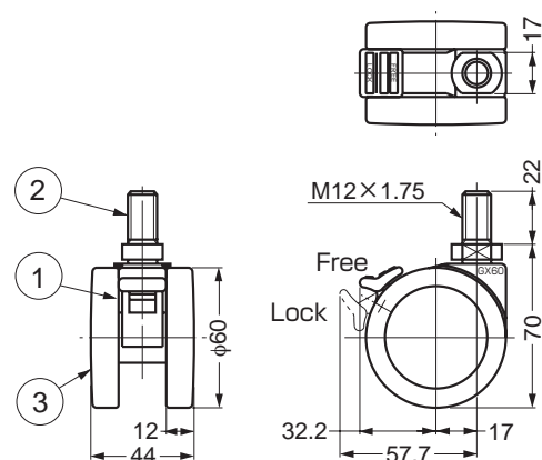
The drawing above show the model with Brake
