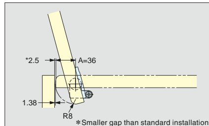
Installation with Rounded Lid Edge
