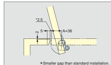
Installation with Inclined Edge
