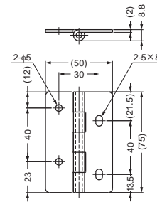
SR75B
