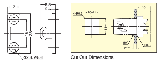
Cut Out Dimensions
