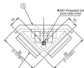
PJ-80AT (For 8mm slot frame)
