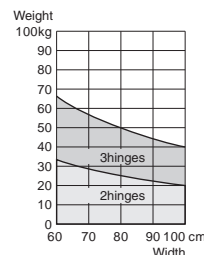
DA180-5934
