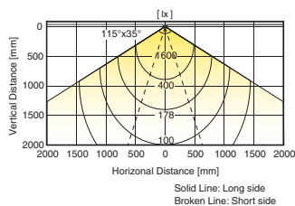
[SL-WPG 2]
