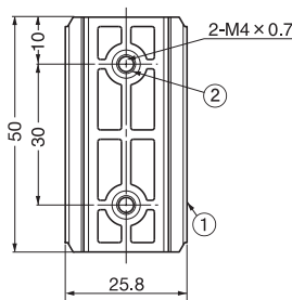
MR-50C
