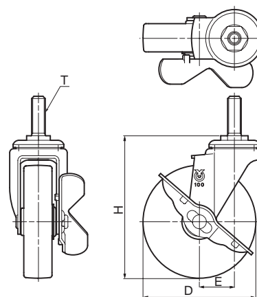
The drawing above show the model with Brake
