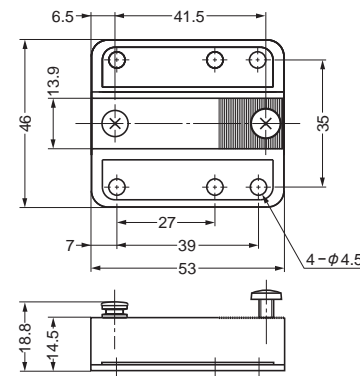
HT-160TZ(Mounting Plate)
