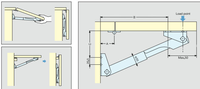
Installation example for 38820-25
