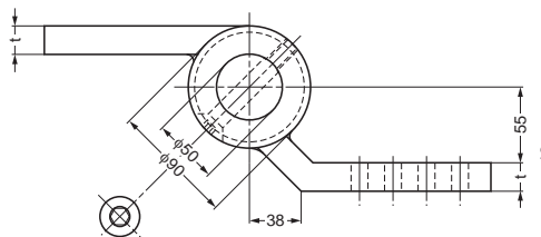
HG-KM19-275, HG-KM20-250
