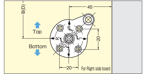
Mounting Plate SDS-A
