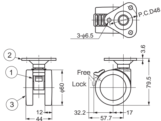
The drawing above show the model with Brake
