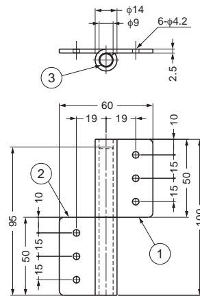
LSX-100R
