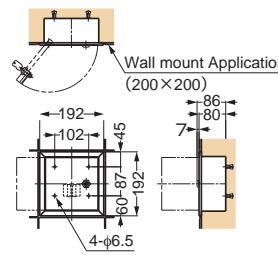
AP-BR060 (Mortise Mount)
