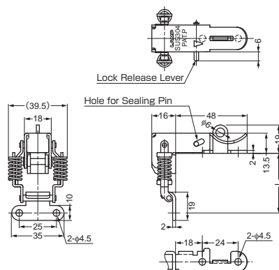
STF-C64A With Spring
