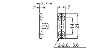
Strike for wood(1)
