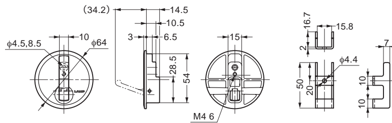
Bracket NF-50 (Option)
