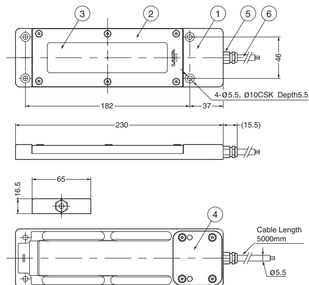
[SL-WPG 1]
