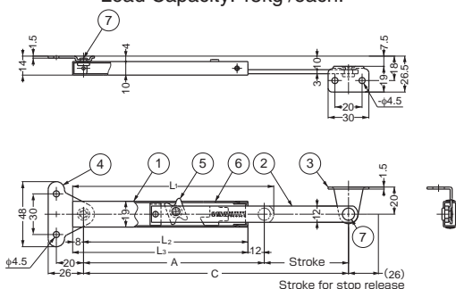
The above dimension for LB-215B and LB-290B. ( ) Dimension...L-290
