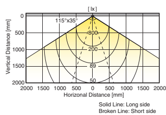
[SL-WPG 1]
