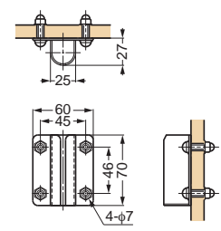
AP-BR061 (Surface Mount)
