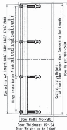
4 Hinges per door ①Damper and Catch Hinges : 3 pcs ②Non Damper and Catch Hinges : 1pc *Please install the ② to the second place from the bottom.
