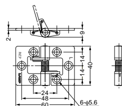
■ Closing Tension(SC type)
