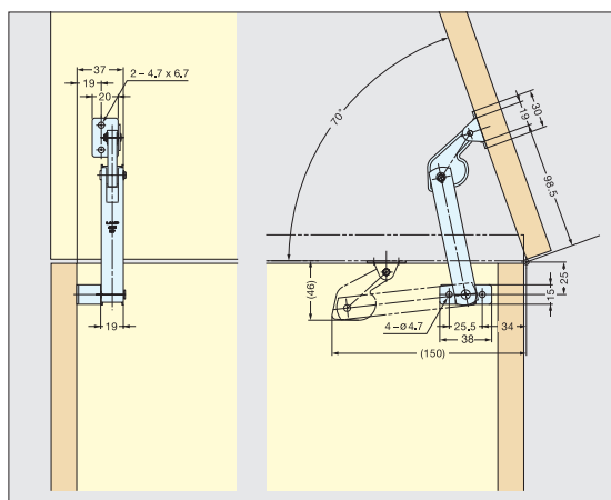
For side mount type
