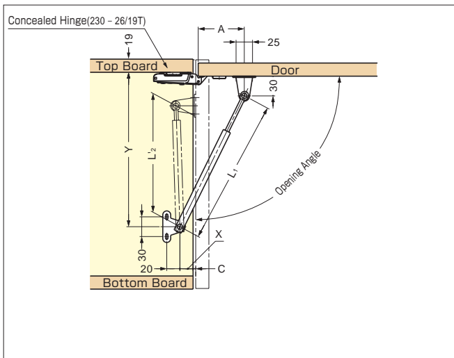
Mounting Example (1) LK-222, LK-335 (Wooden door)
