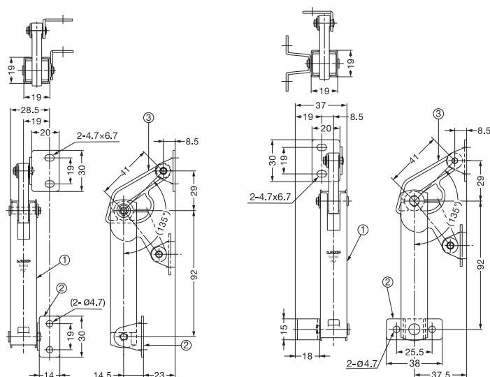
Back panel mount type
