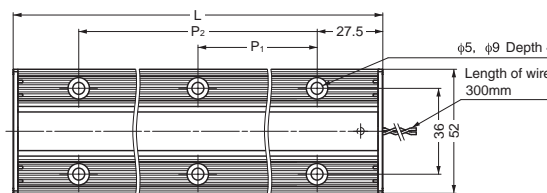
Cover with screw visible
