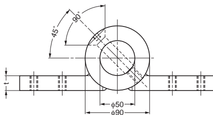
HG-KH19-275, HG-KH20-250
