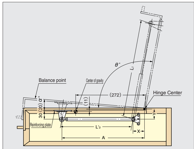
Mounting Example (2) LK-335, LK-380 (Plastic Lid)
