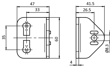
Set Haltewinkel 60 × 47 × 4, D28 Set Mounting Bracket 60 × 47, D28
